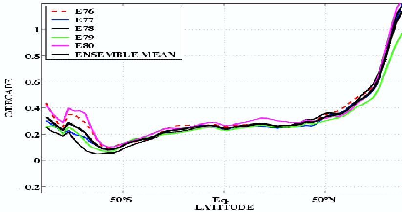
Figure 2. 80-year mean of a five different transient climate change experiments with the Bergen climate model showing the zonal average temperature increase during a time when the \text{CO}_2 forcing is increasing by 1%/year compared to a case when \text{CO}_2 is constant. The ensemble mean is also indicated. Courtesy H. Drange, Bergen Climate Centre.
