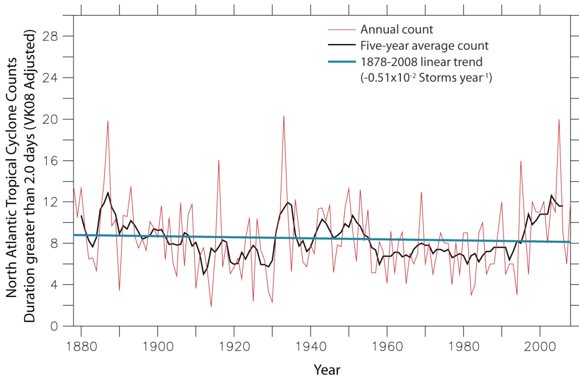
Figure 5: Adjusted frequency (in red) of Atlantic moderate to long-lived tropical cyclones from 1878 to 2008. The black curve is a five-year centered mean and the blue line is the 1878 to 2008 trend.
