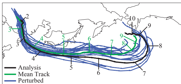
(a) ECMWF - forecast started 1200 UTC 27 Feb 2005
